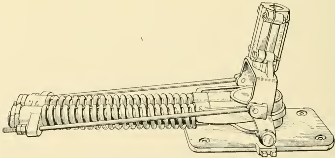
Fig. 102. Trolley Base with Ball-Bearing
